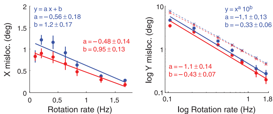
Figure 6. The effect of optic flow speed on X - and Y -mislocalizations, plotted with the same graphical conventions as used in Figure 5 . The logarithm of the Y -mislocalization decreases linearly with the logarithm of the rotation rate, which was expected on the basis of instantaneous velocity summation. However, a significantly negative dependence of X -mislocalization on rotation rate was also found, which is inconsistent with the idea that the X -mislocalization depends exclusively on gaze displacement.
